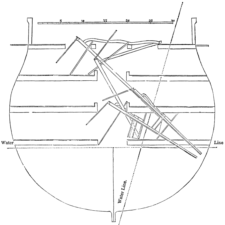
Arrangement of the Pumps, in heaving down.
