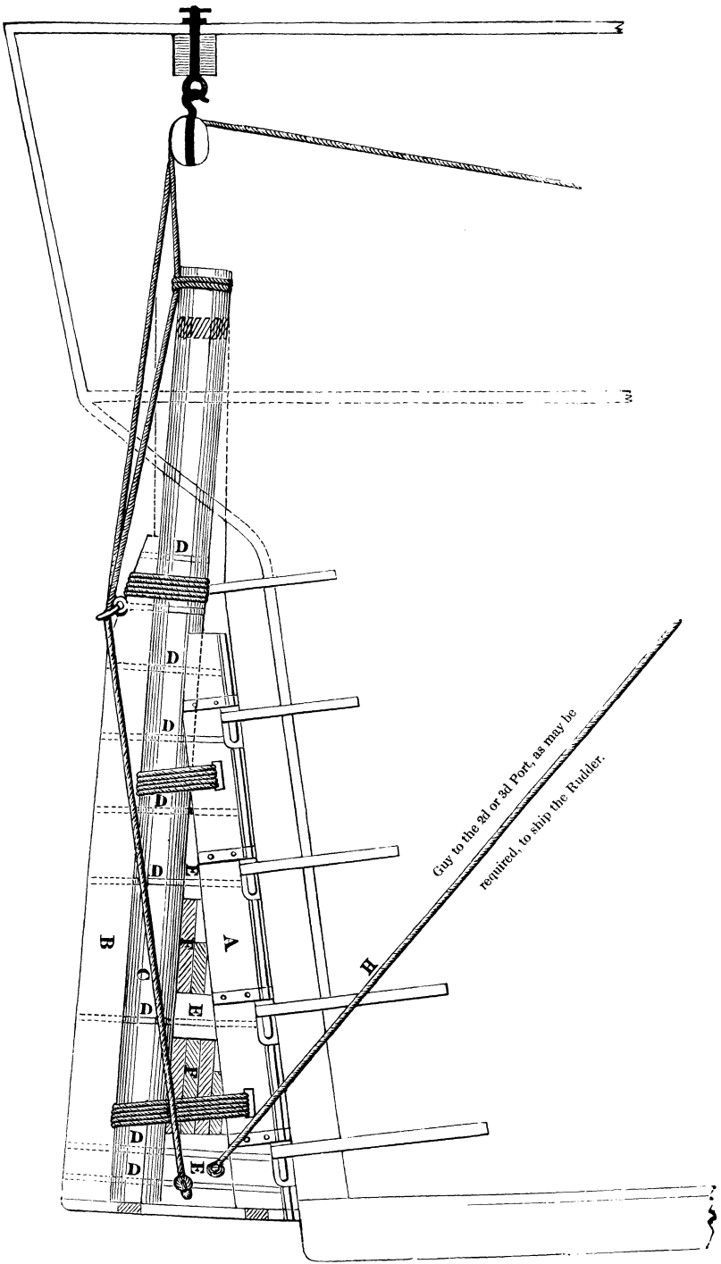
Representat.on of a Temporary Rudder.
