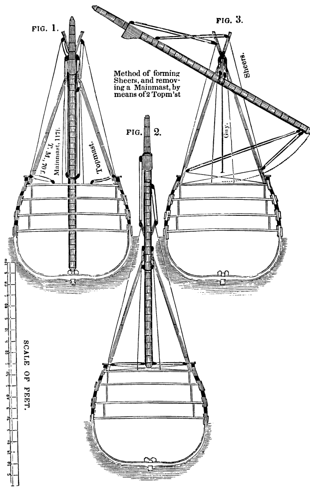
Masting and Dymasting.
