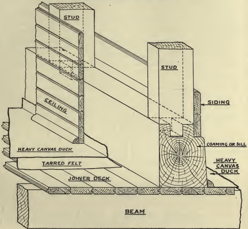
FIGURE-175 SHOWING COAMING AS ON JOINER DECK
