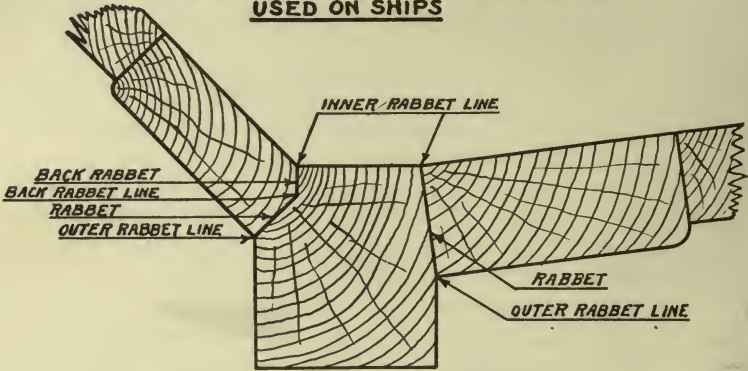
FIGURE-28 AS ON KEEL
