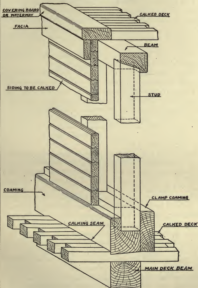
FIGURE-172 SHOWING SECTION OF HEAVY WEATHER BULKHEAD AS USED FOR POOP BRIDGE AND FORECASTLE.
