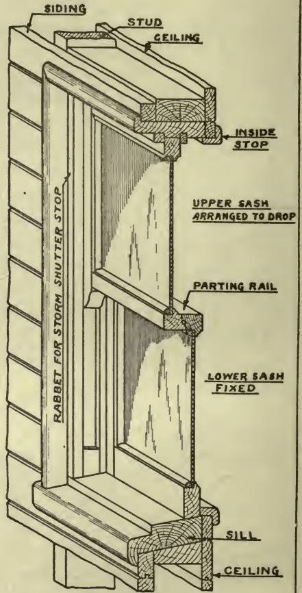
FIGURE-188 SHOWING SASH AND FRAME BUILT AND SET IN PLACE AS A UNIT
