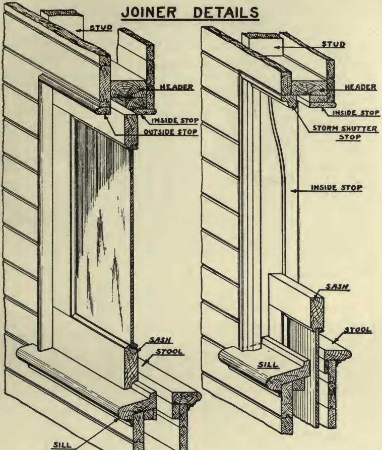
FIGURE-186 SHOWING TRIM WITH STORM SHUTTER STOP
