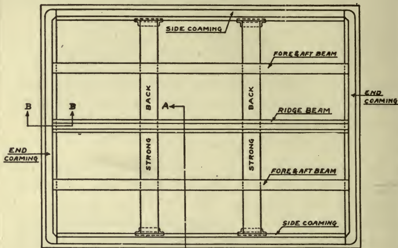
PLAN OF HATCH WITH COVERS REMOVED
