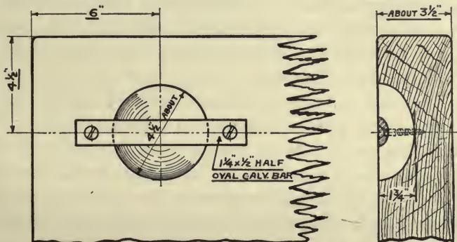
FIGURE-148 ENLARGED DETAIL OF CORNER SHOWING PROPORTIONS OF HAND HOLD
