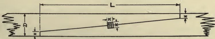
FIGURE-35 KEY LOCKED SCARF
