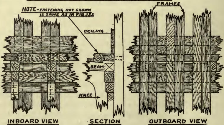
FIGURE-133 AS ON WEATHER DECK IN WAY OF BRIDGE ALSO AS ON TWEEN DECKS
