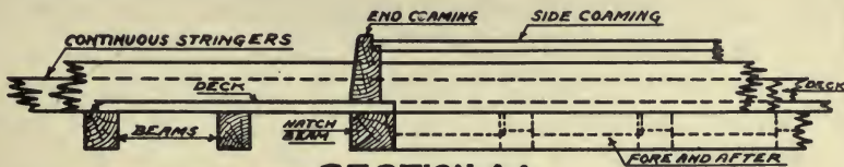
SECTION-A-A SHOWING COAMING AND DECK STRINGERS AS ON WEATHER DECK
