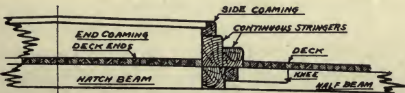
SECTION-B-B SHOWING WEATHER DECK COAMING AND STRINGERS ALSO TYPICAL SHAPE OF END COAMING FOR ALL SHIPS
