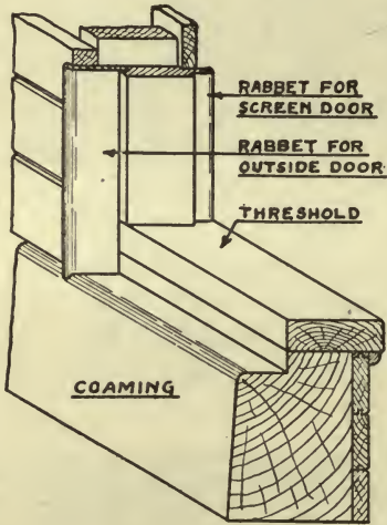
FIGURE-187 SHOWING DOOR FRAME AND TRIM WHERE INBOARD SCREEN DOOR IS FITTED
