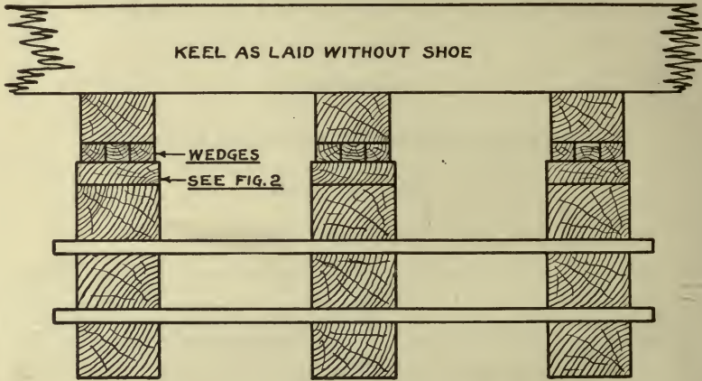
FIGURE-1 ELEVATION
