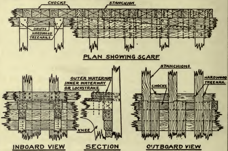
FIGURE-132 AS ON WEATHER DECK IN WAY OF BULWARK
