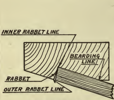
FIGURE-30 AS ON RIM
