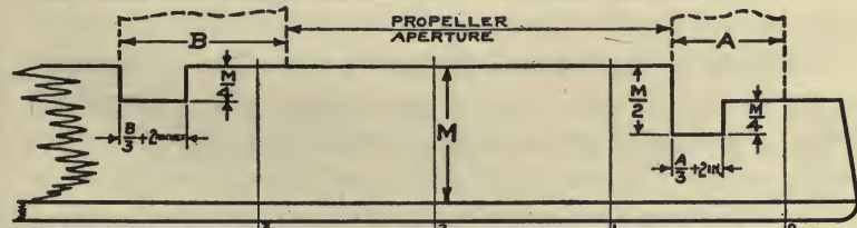
FIGURE-15 FOR SINGLE SCREW SHIPS WITH WOOD RUDDERS
