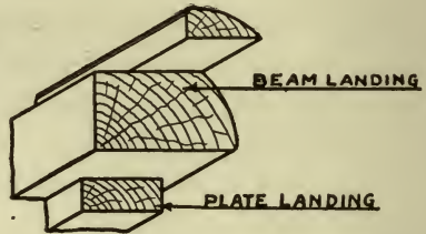
FIGURE-180 UPPER END OF CORNER POST
