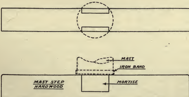
FIGURE-171 SHOWING ONE FORM OF MORTISE USED IN STEPPING MASTS
