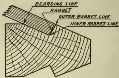
FIGURE-29 AS ON STEM
