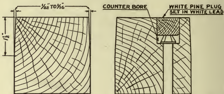
FIGURE-141 SECTION OF WEATHER DECKING
