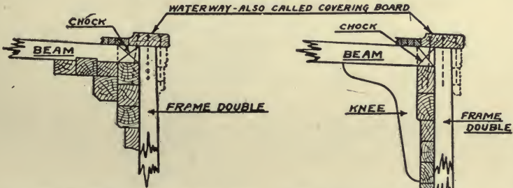
FIGURE-135 AS ON SHELTER DECK
