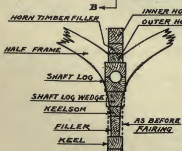
SECTION-B-B FIGURE-63
