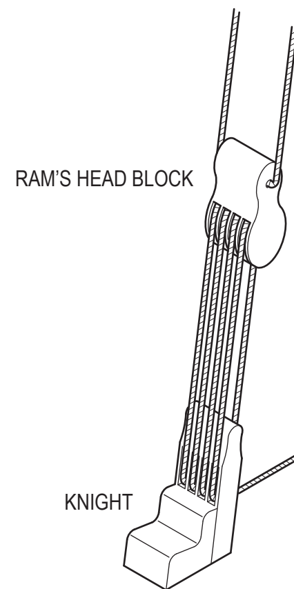
TYPICAL KNIGHT & BLOCK RIGGING
