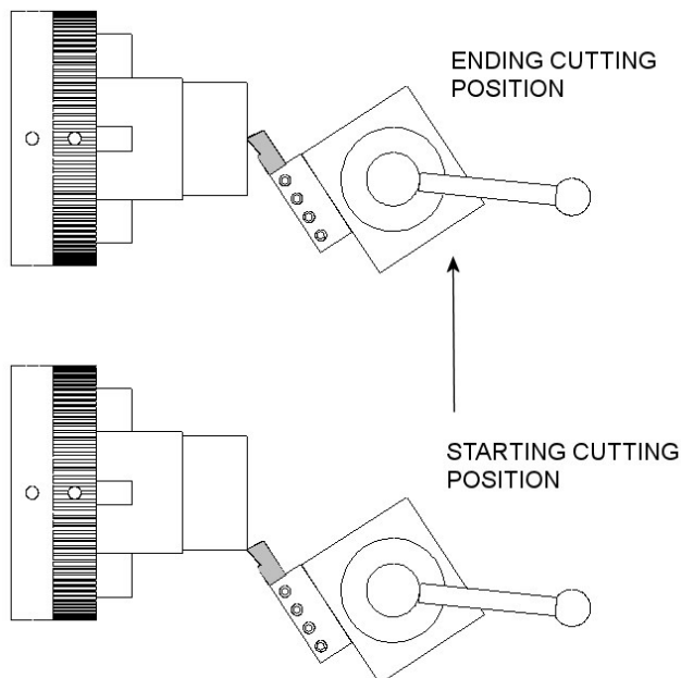
NOTE THE DIFFERENT ANGLE OF CUTTING TOOL PROPER TOOL POSITION FOR FACING STOCK USE THE "Y" ADJUSTMENT KNOB TO MAKE CUT
