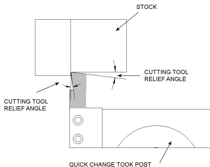
A 2D view showing looking down on your Tool Post and Cutting Tool showing the relationship of the Tool as it is positioned to the Stock. The Cutting Tool is usually at 90° degrees to the material you are cutting into. Take note of the “Relief” angles. This is very important so that the cut material can escape from the cut, otherwise, the tool will bind, heat up and cause chatter and uneven cuts.
