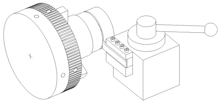
PARTING TOOL CUTTING THROUGH STOCK
