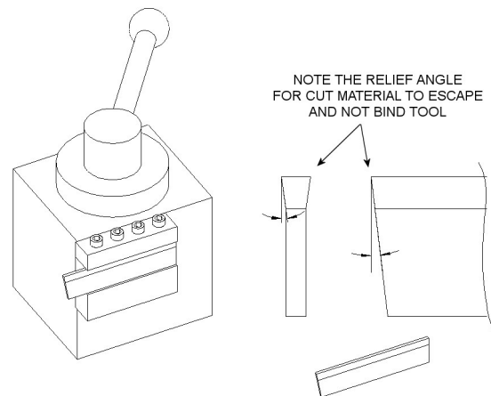
PARTING CUTTING TOOL DETAIL
