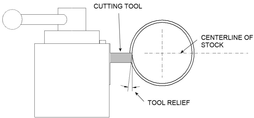
SIDE VIEW LOOKING INTO STOCK. NOTE THE CUTTING TOOL IS AT CENTER OF STOCK.
